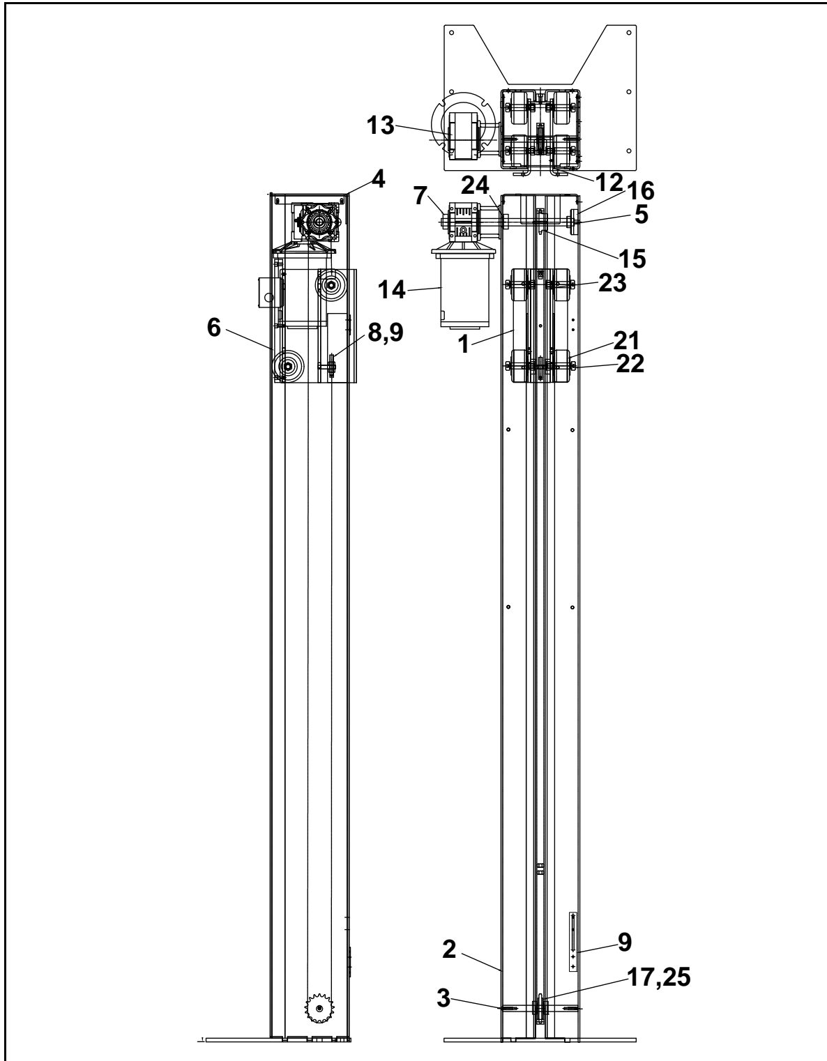
Figure 11-2. EZ/Pro Top Drive Tower Assembly
