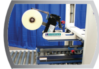
Tip-up tape head simplifies roll replacement
